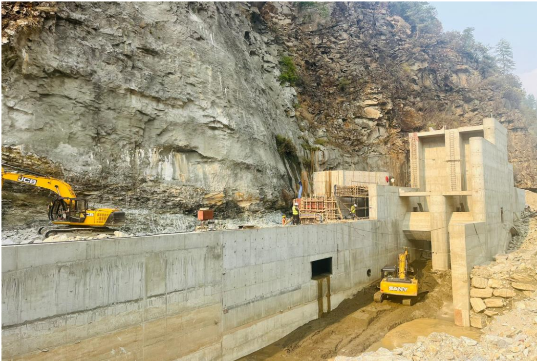
Undersluice Area
