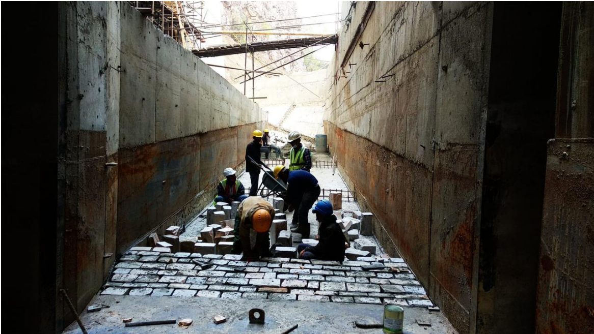
Hardstone Lining at Undersluice
